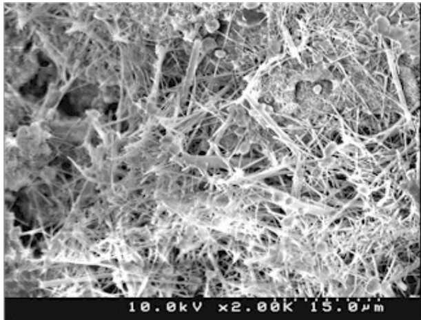
Fig 2. Microstructure on Sample of Xypex Admix Modified Concrete; Magnification x 2000
