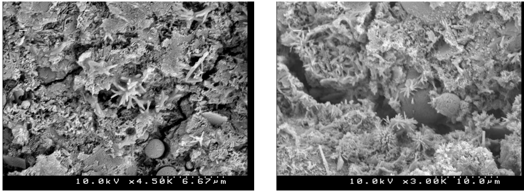
Fig 3. Microstructure on Sample of Penetron Modified Concrete; Magnification x 4500 (left) and x 3000 (right)
