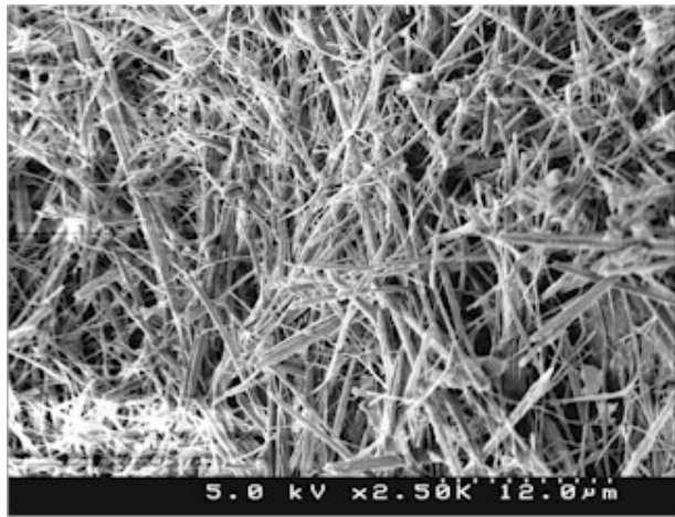
Fig 1. Microstructure on Sample of Xypex Admix Modified Concrete; Magnification x 2500
